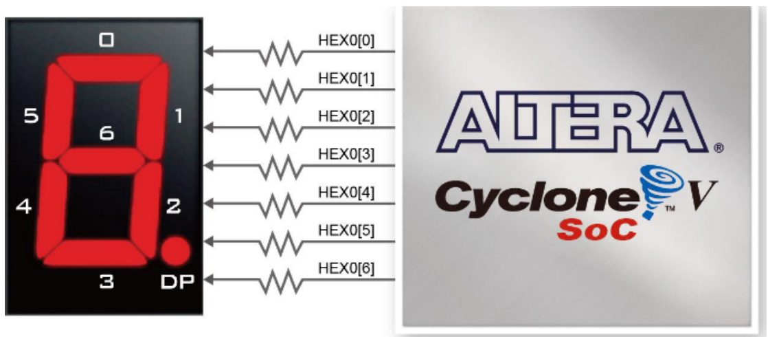
Figure 2: The connections between the common anode 7-segment display HEX0 and the FPGA on the DE1-SoC board.
