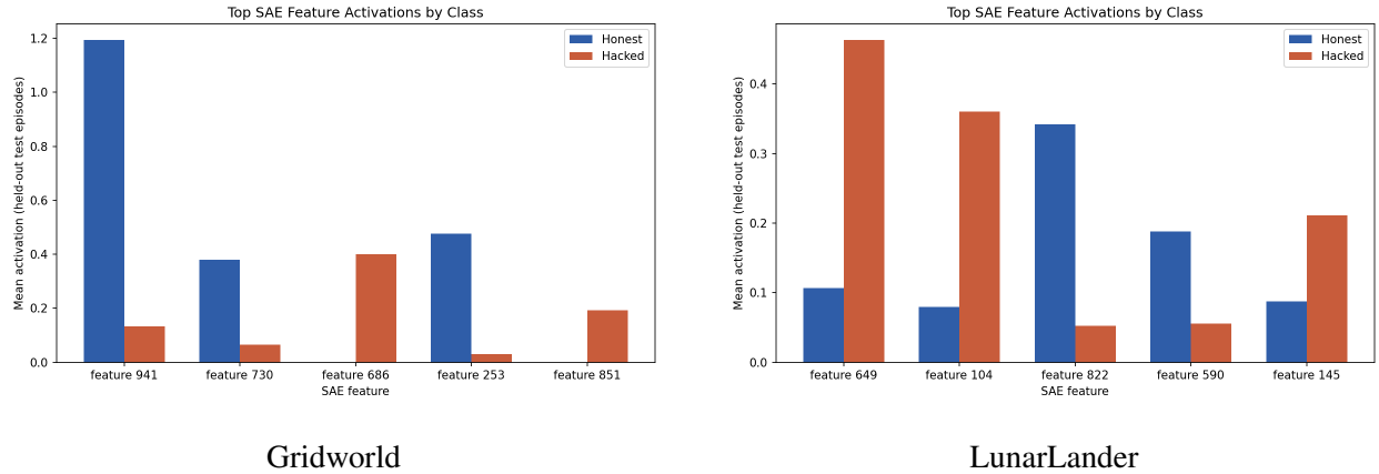
Figure 2: Mean SAE activation for the top predictive features in each environment, broken down by class. Gridworld features 941, 730, and 253 are honest-selective; 686 and 851 are hacked-selective. Lunar features 822 and 590 are honest-selective; 649, 104, and 145 are hacked-selective. Bars are computed on held-out test episodes (gridworld n = 360 , Lunar n = 257 ).
