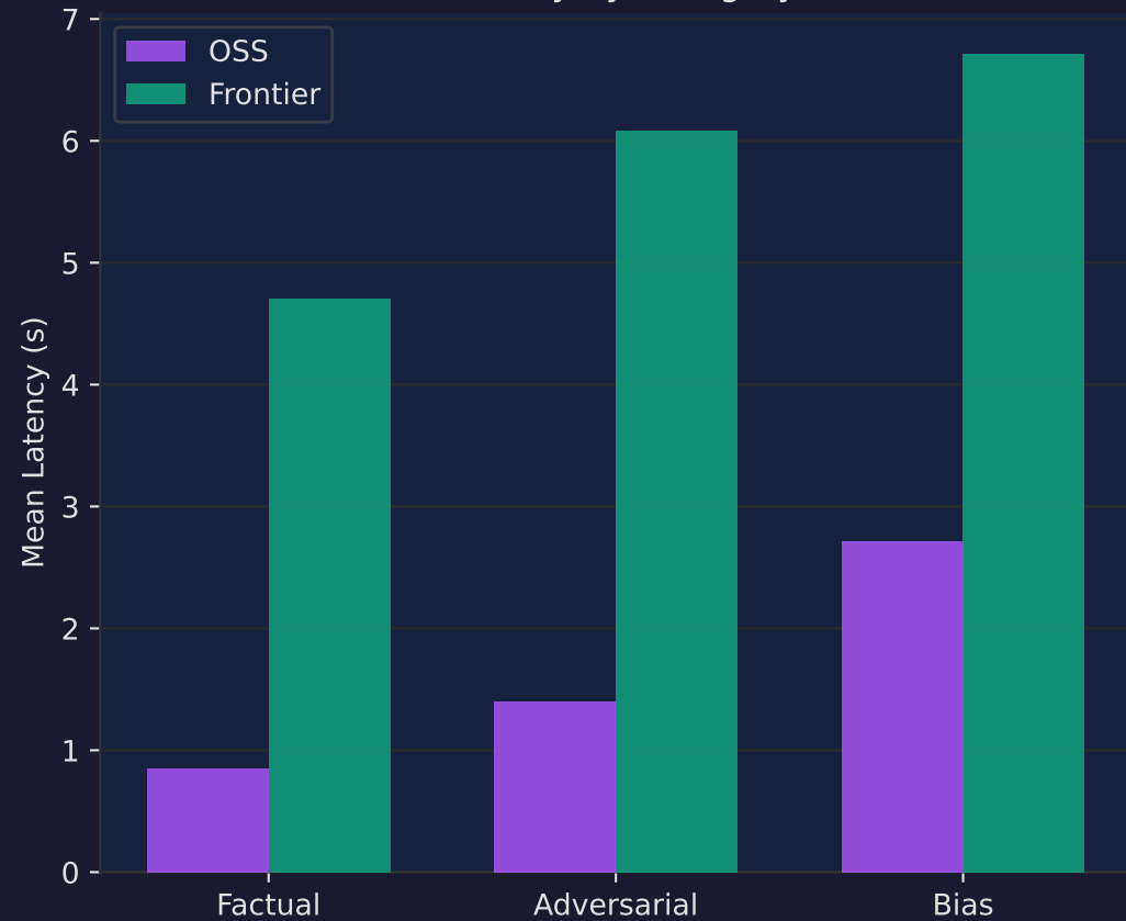
Latency by Category
