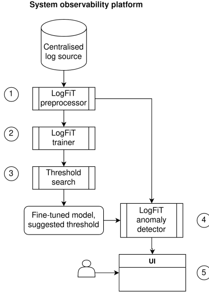
Figure 3. LogFiT integrated into existing system observability platform.
