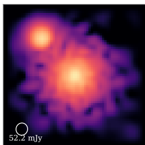
Gaussian envelope
