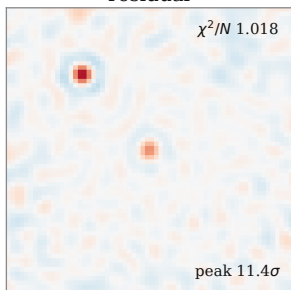
residual
