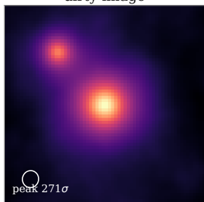
dirty image
