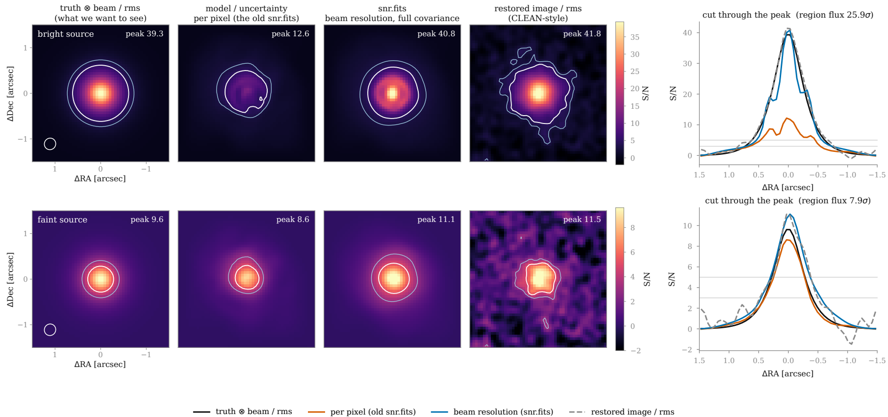
Mock exponential disc, 4800 visibilities: contours at S/N 3 and 5; one colour scale per row
