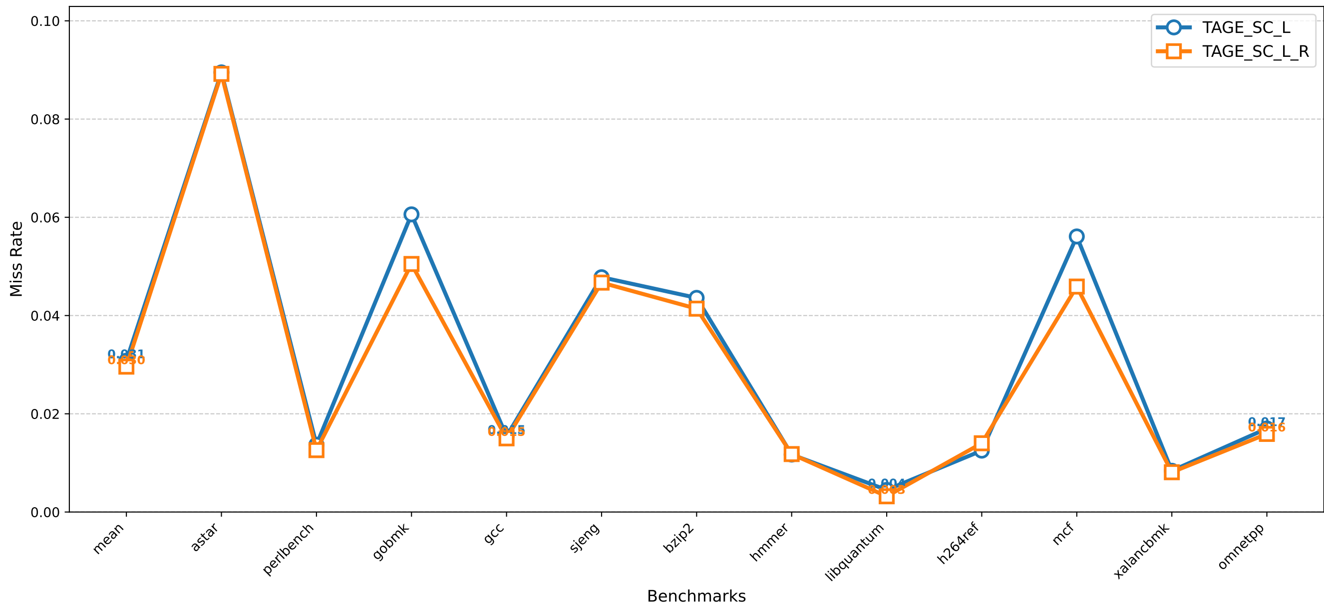
Miss Rate Comparison: TAGE_SC_L vs TAGE_SC_L_R
