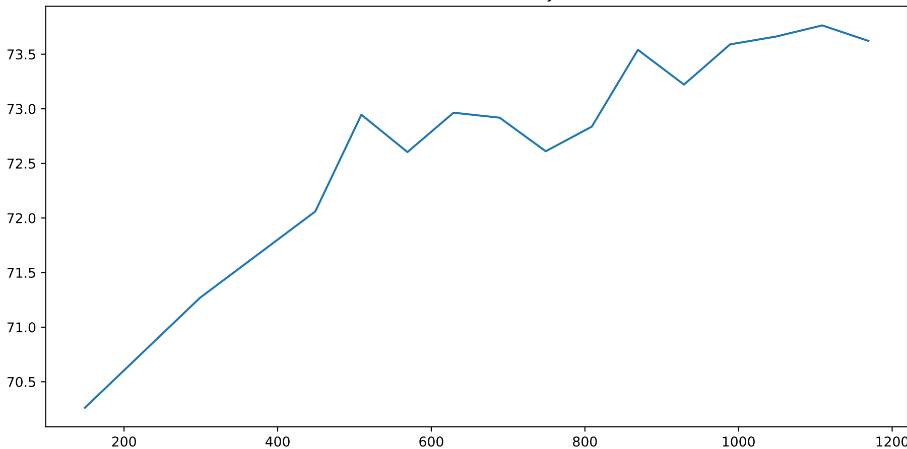
Regularization Losses
