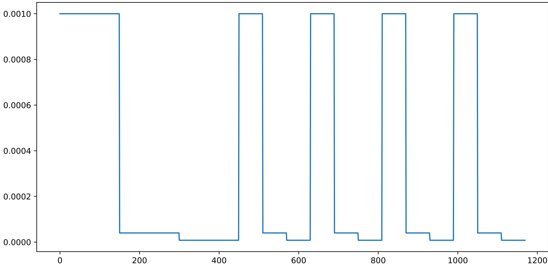
Learning Rate
