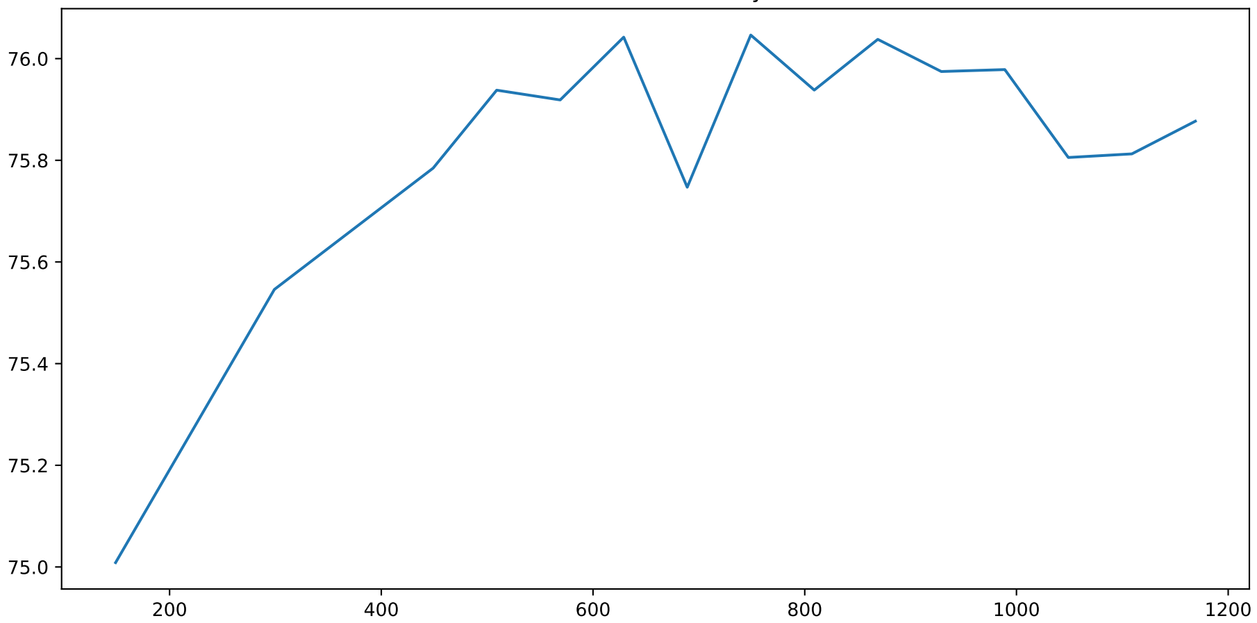
Regularization Losses
