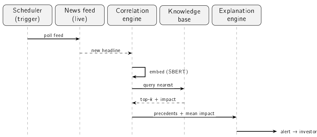
Figure 4.4: The news trigger as an interaction over time. Solid arrows are calls, dashed arrows are returns; time runs downward. The correlation engine orchestrates the work: it embeds the headline, consults the knowledge base, and assembles the retrieved precedents and their measured impact, before the explanation engine renders and delivers the alert. This complements the data-flow view of Figure 4.3.
