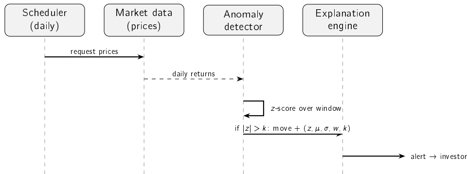
Figure 4.6: The market-movement trigger as an interaction over time. Solid arrows are calls, dashed arrows are returns; time runs downward. The detector standardises the latest return against its rolling window and forwards the move (with the z-score, window, threshold, mean and standard deviation) to the explanation engine only when the threshold is exceeded. This complements the data-flow view of Figure 4.5.
