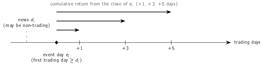
Figure 3.5: How impact is measured. The news date d_i may fall on a non-trading day; the event day e_i is the first trading day on or after it. The return is then accumulated forward from the close of e_i over +1, +3 and +5 trading days. Only post-event days are used, so no future information enters.
