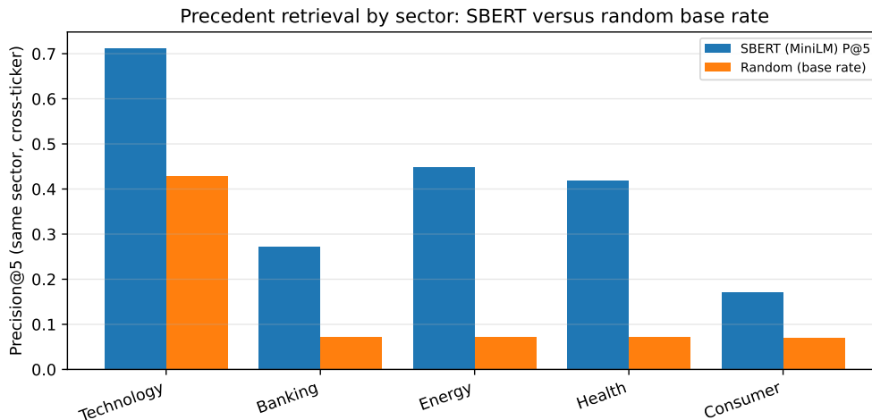
Figure 5.7: Precision@5 per sector against the random base rate. Retrieval exceeds the base rate in every sector; the gap (lift) is largest for energy and health, whose vocabulary is most distinctive, and smallest for the broad consumer sector.
