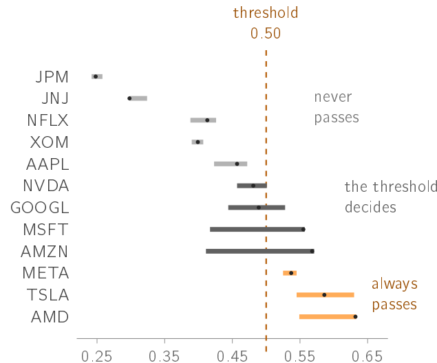
Figure 5.15: Range of all the scores the model assigned to each company in production, with the median marked. The light bars never reach the threshold, the dark ones cross it and the orange ones sit always above it. Eight of the twelve companies lie entirely on one side, which means that for those the decision was taken before the headline was read.
