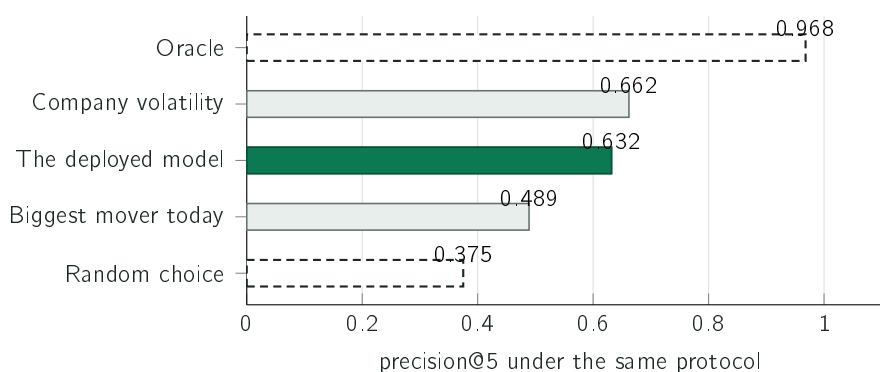
Figure 5.18: Five selection policies over the same test block. Random choice serves as the reference; the oracle is a theoretical maximum that is not usable, obtained with knowledge of the answers. All of them choose knowing the complete day, so each value is an upper bound on what the same rule would obtain deciding minute by minute.
