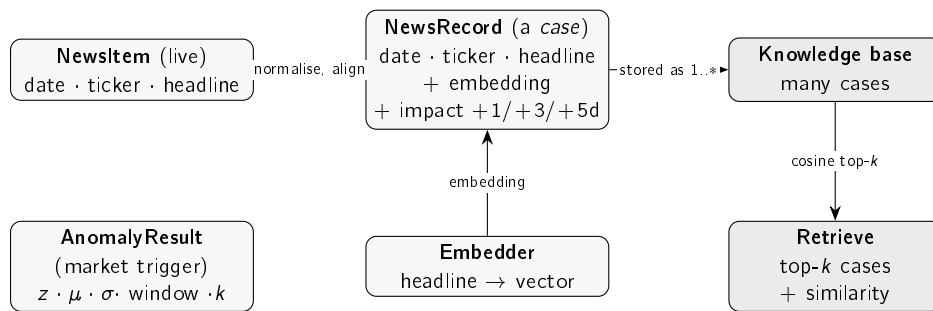
Figure 4.3: The objects InvestiGator works with. A live NewsItem and a historical NewsRecord share the same schema (date, ticker, headline); a NewsRecord is a case , adding the headline's embedding and its measured post-event impact. The Embedder produces those vectors; the Knowledge base holds many cases; a query headline retrieves the top- k most similar cases with their similarity scores. The market trigger produces a separate AnomalyResult .
