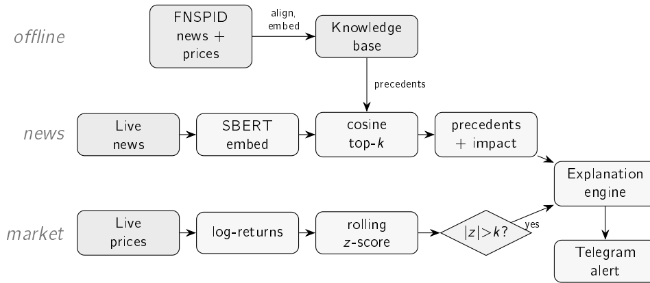
Figure 4.4: The end-to-end flow of InvestiGator as one connected pipeline. Offline (top), FNSPID news is aligned to prices and embedded into the knowledge base. The news trigger (middle) embeds an incoming headline, finds its nearest precedents in the knowledge base and attaches their observed impact; the market trigger (bottom) turns live prices into a z-score and fires only when it exceeds the threshold. Both paths converge on the explanation engine, which delivers one explained alert through Telegram. This is the simplified view; the complete pipeline, with every decision gate and its live configuration value, is Figure A.1 in Appendix A.
