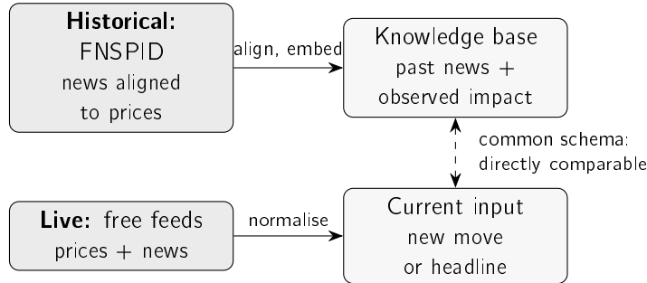
Figure 3.1: The two data layers. The historical layer turns the FNSPID corpus into a knowledge base of past news and its observed price impact; the live layer normalises real-time prices and news into the same fields, so a current event can be compared directly against the precedents.
