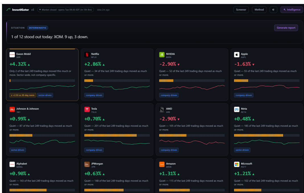
Figure 4.6: The public interface (a genuine screenshot, not a mockup), opening surface, captured from the deployed system during live operation. One card per company, ordered by how rare the day was, none privileged. Every card states its verdict in words and then evidences it with a count rather than asserting it, including when the answer is that nothing happened: Tesla, at +0.70%, reads “201 of the last 249 trading days moved as much or more”. Rarity appears twice, as that sentence and as a strip of marks, so companies can be compared without reading a number — Exxon Mobil, the only flagged name, shows a single lit mark against Tesla’s near-full strip. The attribution line names the driver in words, and the header carries the market’s state and the age of the data, both of which are required because the numbers are those of the last completed session and a reader has no other way to know it.
