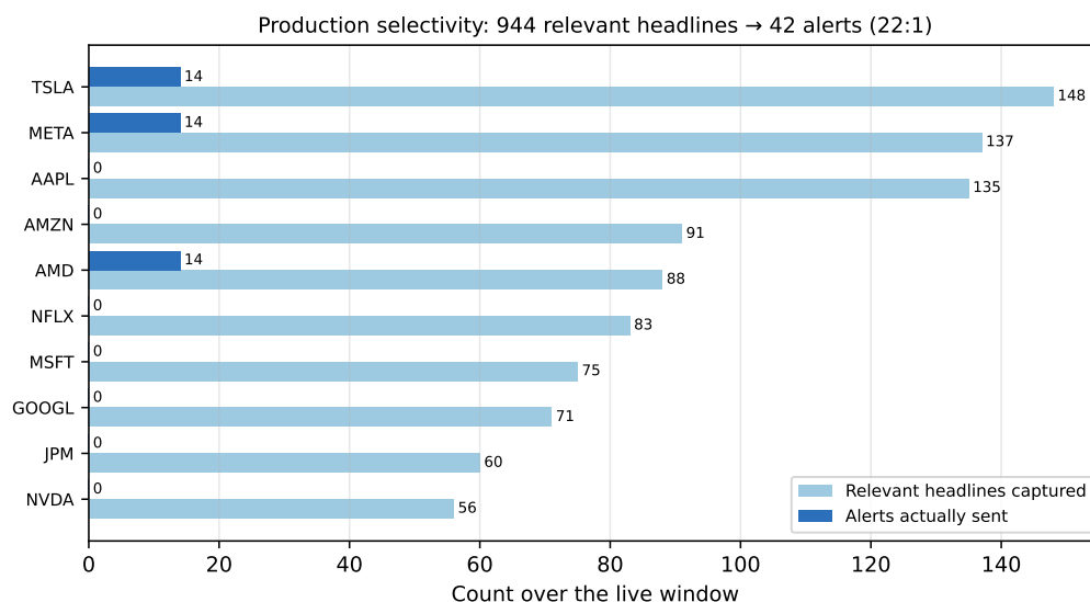
Figure 4.8: Production selectivity over the first five live days: relevant headlines captured (light) versus alerts actually sent (dark), per watchlist ticker. All counts are real, read from the shared data branch; the gap between the two bars is the work of the quality gates of Table 4.8.
