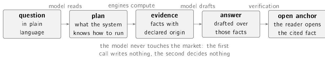
Figure 4.13: The two calls to the language model are separated on purpose. The first translates a human sentence into a plan the system knows how to run and writes no text. The second drafts over facts that already exist and decides nothing. Between them, the engines described in this chapter produce the evidence, and each fact arrives with its origin declared. The final verification refuses any sentence whose number does not belong to the fact it cites, and that is what lets the reader open the anchor and confront the claim with what supports it.
