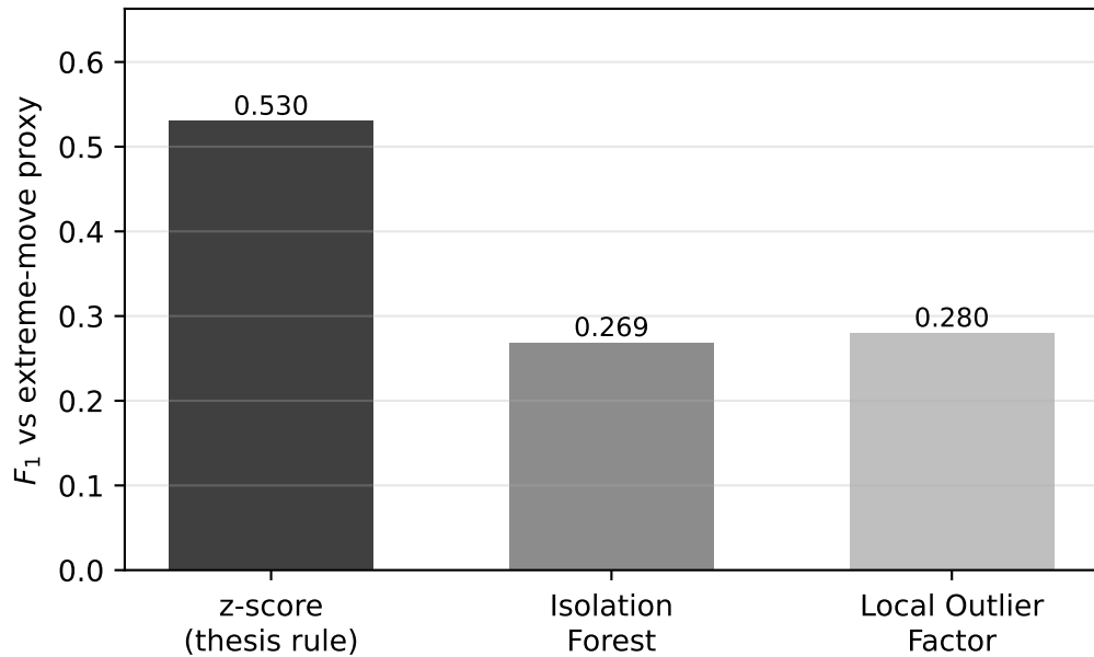
Detector (same causal features)
