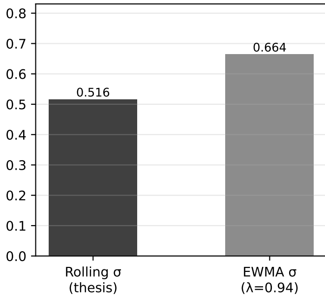
Volatility estimator
