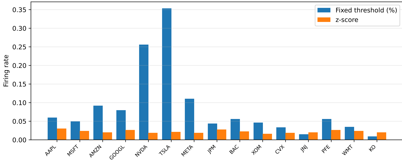
Firing rate per ticker: fixed threshold versus z-score
