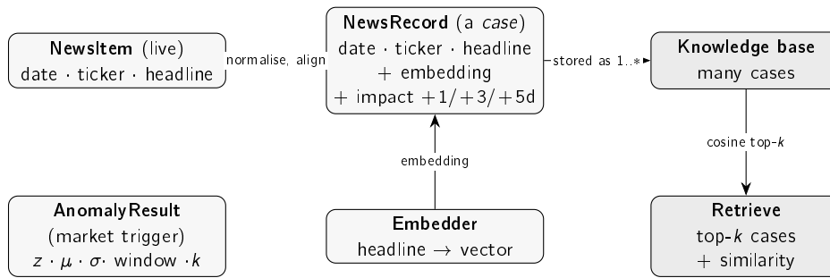
Figure 4.2: The objects CLARION works with. A live NewsItem and a historical NewsRecord share the same schema (date, ticker, headline); a NewsRecord is a case, adding the headline's embedding and its measured post-event impact. The Embedder produces those vectors; the Knowledge base holds many cases; a query headline retrieves the top- k most similar cases with their similarity scores. The market trigger produces a separate AnomalyResult .
