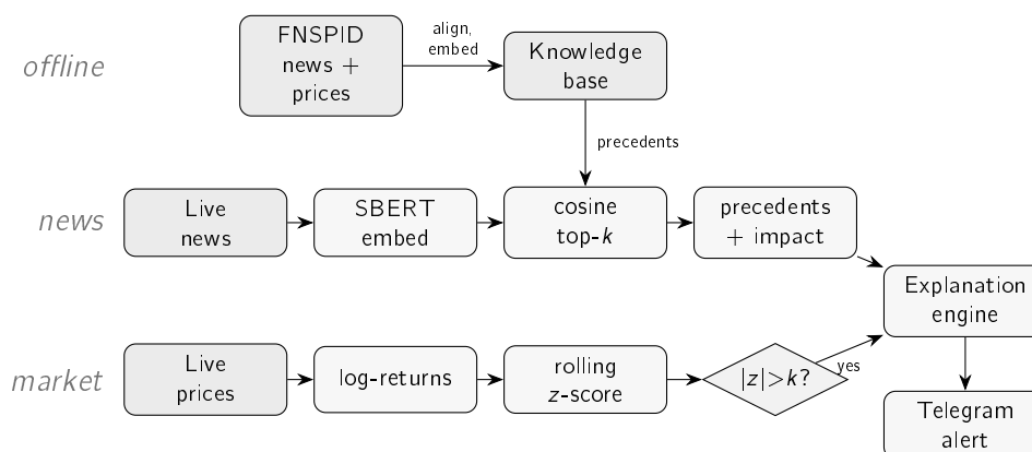
Figure 4.3: The end-to-end flow of Clarion as one connected pipeline. Offline (top), FNSPID news is aligned to prices and embedded into the knowledge base. The news trigger (middle) embeds an incoming headline, finds its nearest precedents in the knowledge base and attaches their observed impact; the market trigger (bottom) turns live prices into a z-score and fires only when it exceeds the threshold. Both paths converge on the explanation engine, which delivers one explained alert through Telegram.
