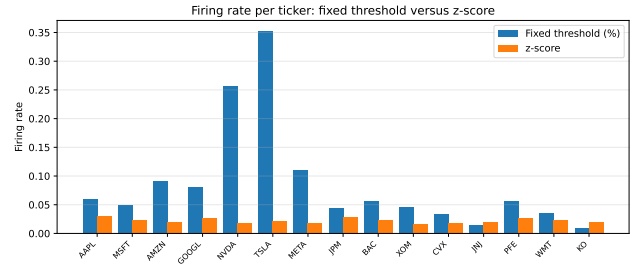
Fig. 1. Firing rate per ticker: a fixed percentage threshold varies dramatically with each stock’s volatility, while the volatility-normalised z -score is stable across all tickers.
