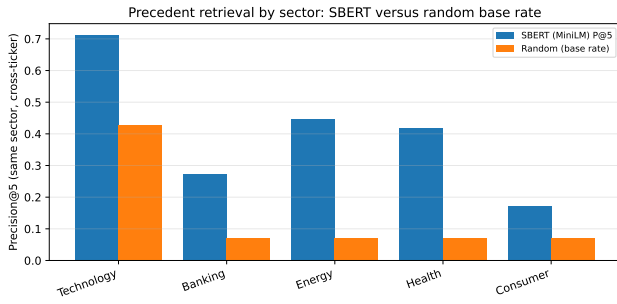
Fig. 2. Per-sector cross-ticker precision@5 against the random base rate. Retrieval beats the base rate in every sector; the lift is largest where the domain vocabulary is most distinctive.
