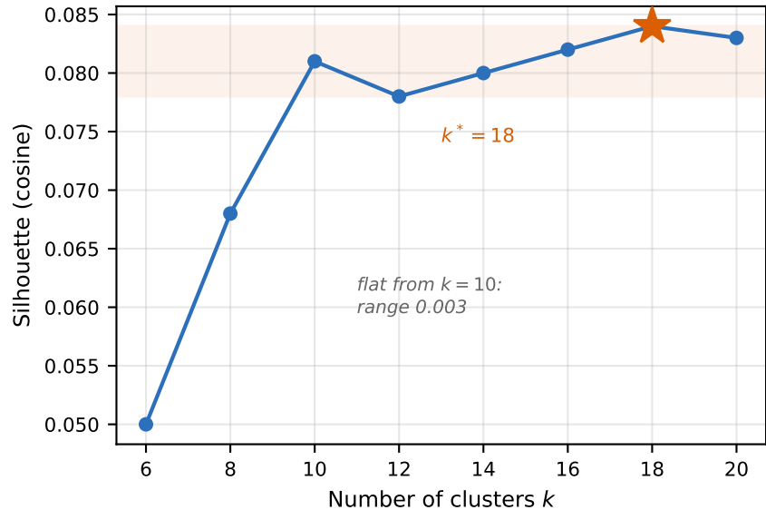
Choosing k : weakly determined
