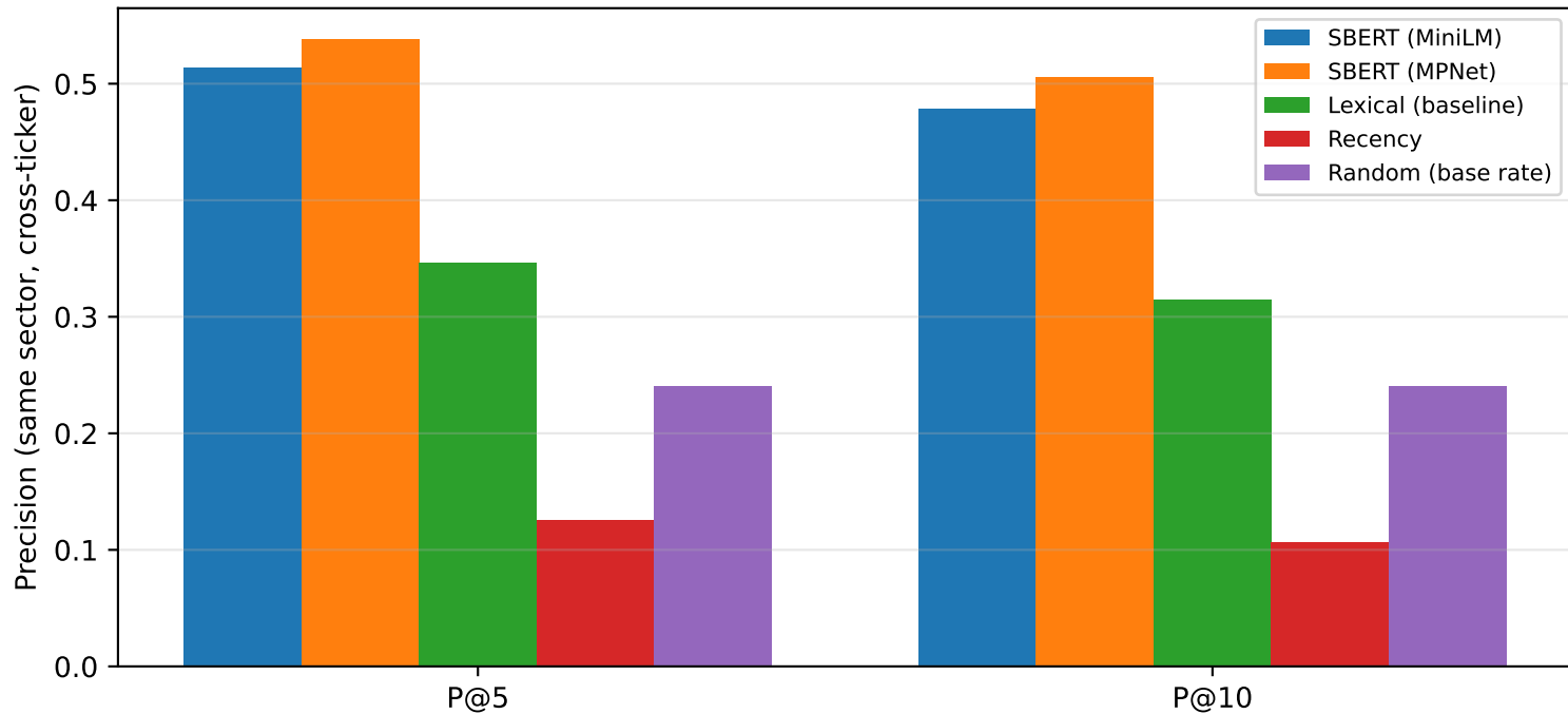
Precedent retrieval: SBERT versus baselines
