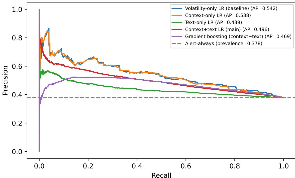
Materiality triage — PR curves (test)
