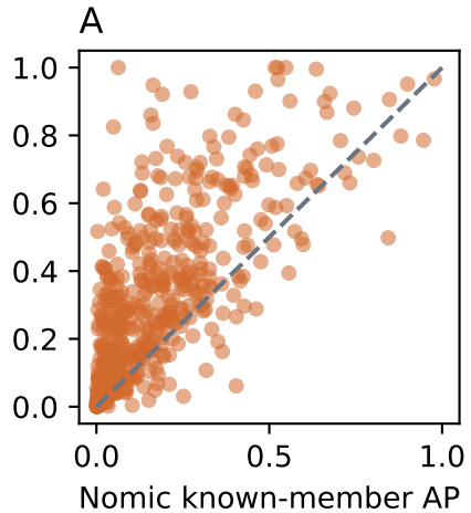
ChEmbed-progressive known-member AP
