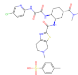
Edoxaban Tosylate
