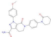
Apixaban
