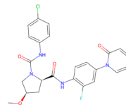
Eribaxaban
