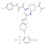
Edoxaban tosylate monohydrate
