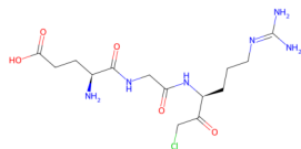
H-Glu-Gly-Arg-chloromethylketone
