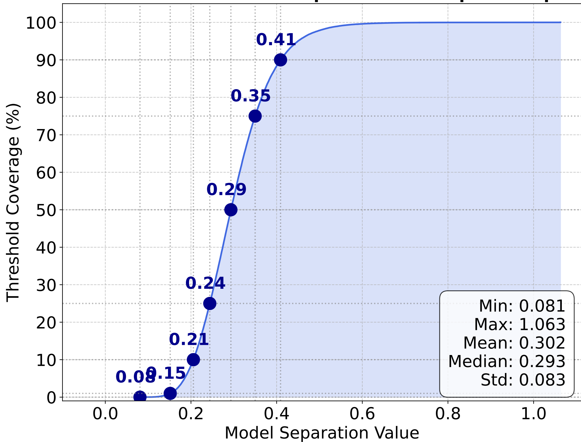
Cumulative Distribution of Computed Model Separation per Path
