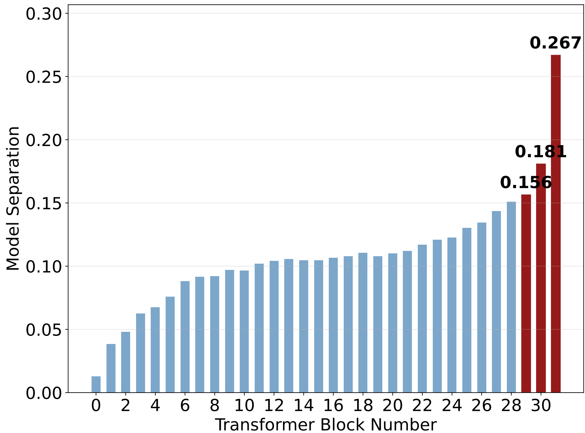
Model Separation Values Across Transformer Blocks
