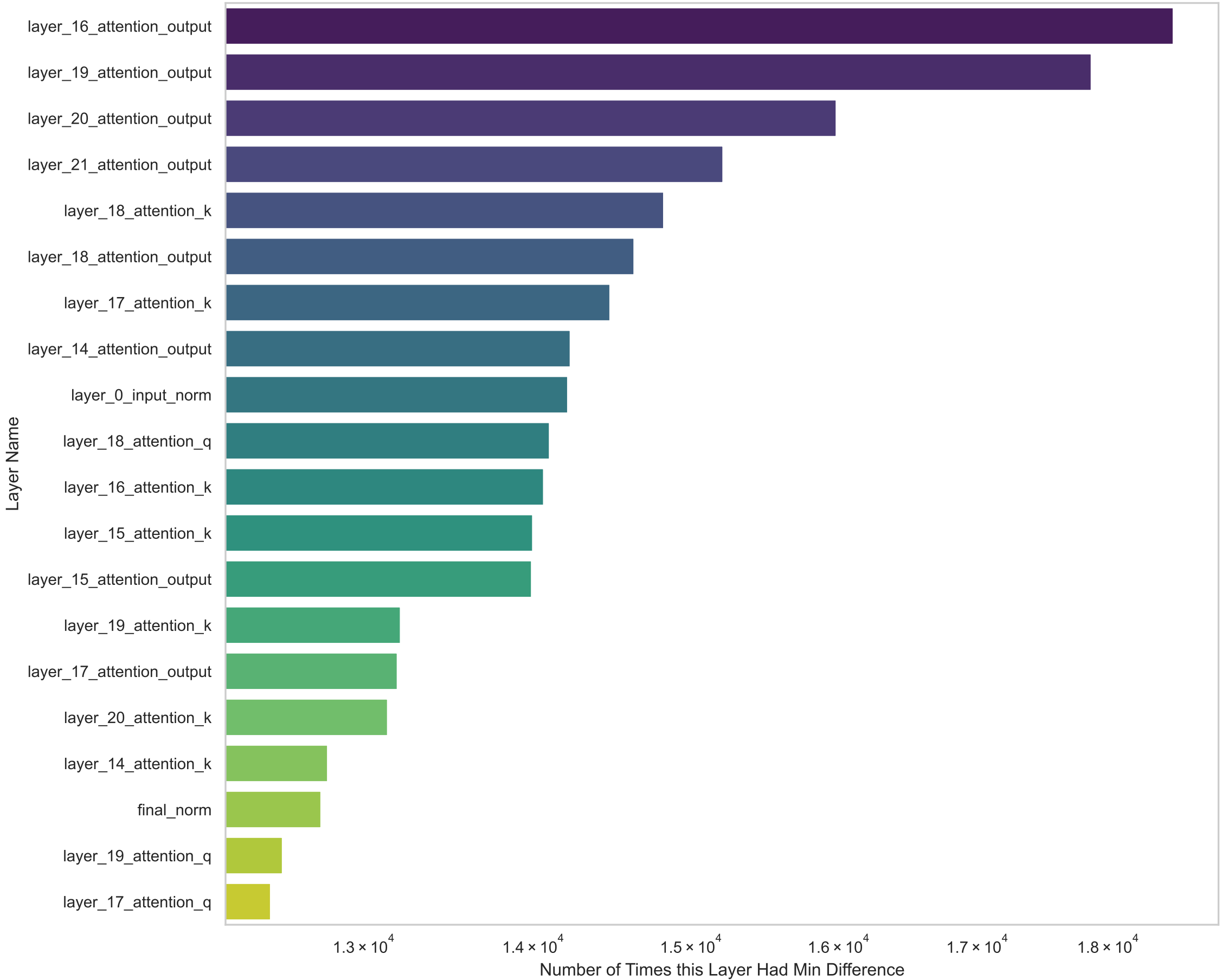
Top 20 Most Vulnerable Layers
