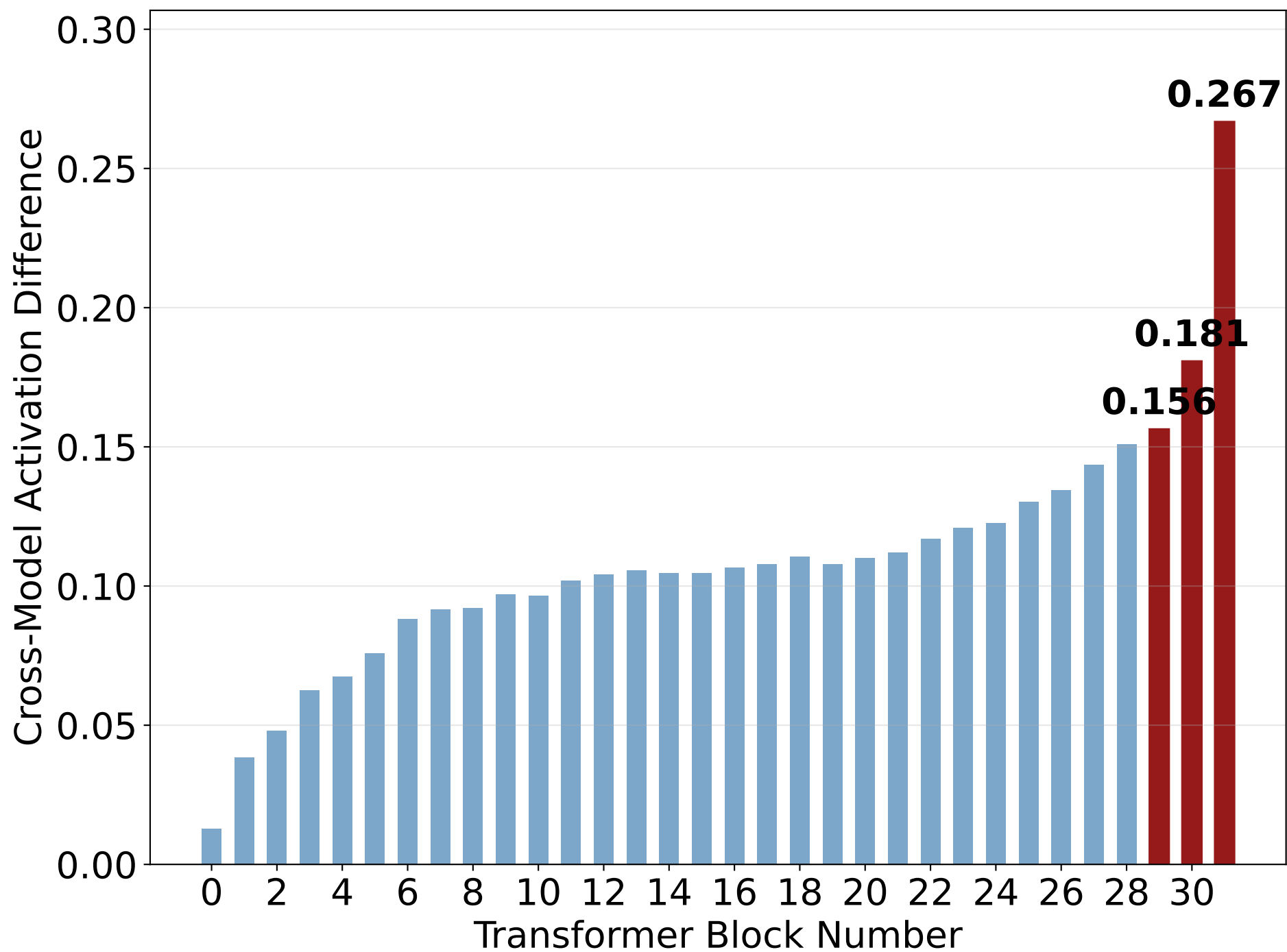
Cross-Model Activation Differences Across Transformer Blocks
