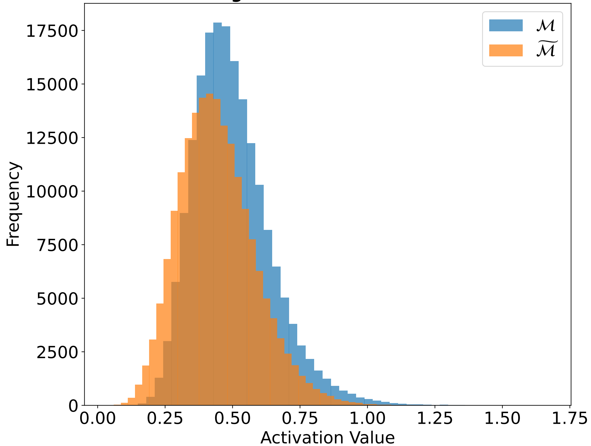
Histogram of Activation Values
