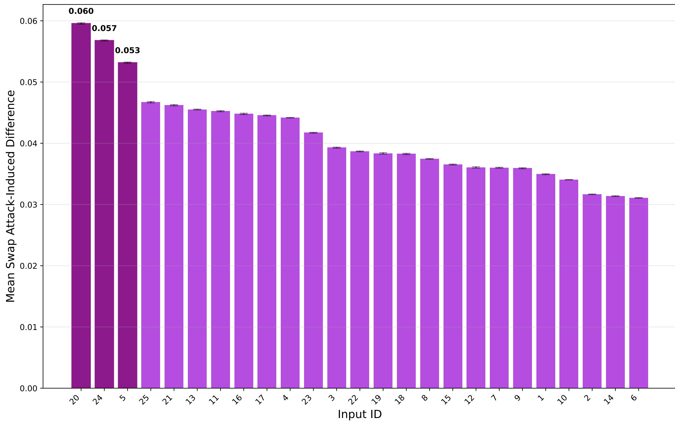
Swap Attack Effectiveness Per Input Prompt
