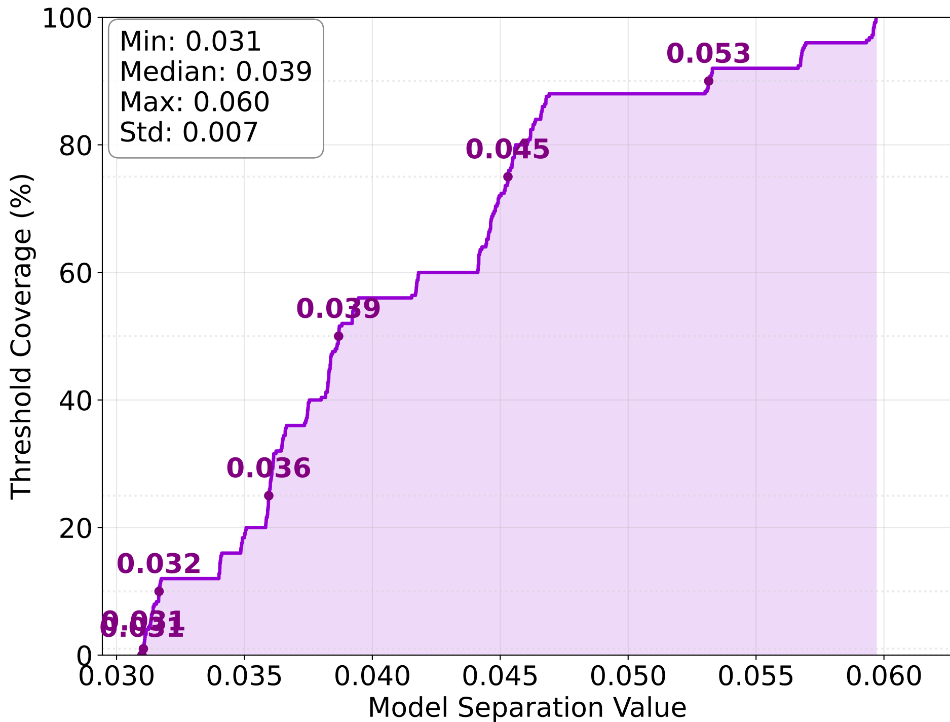
Swap Attack Impact Distribution: Malicious Logit Injection Analysis
