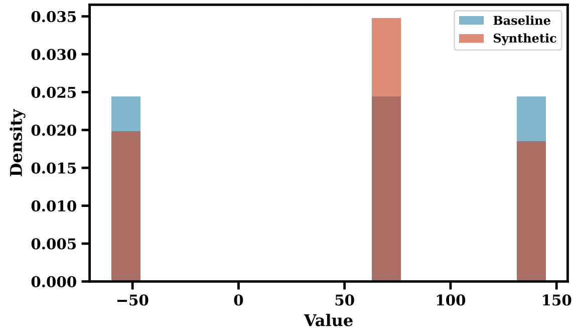
Test Temperature (F) KS p=0.852
