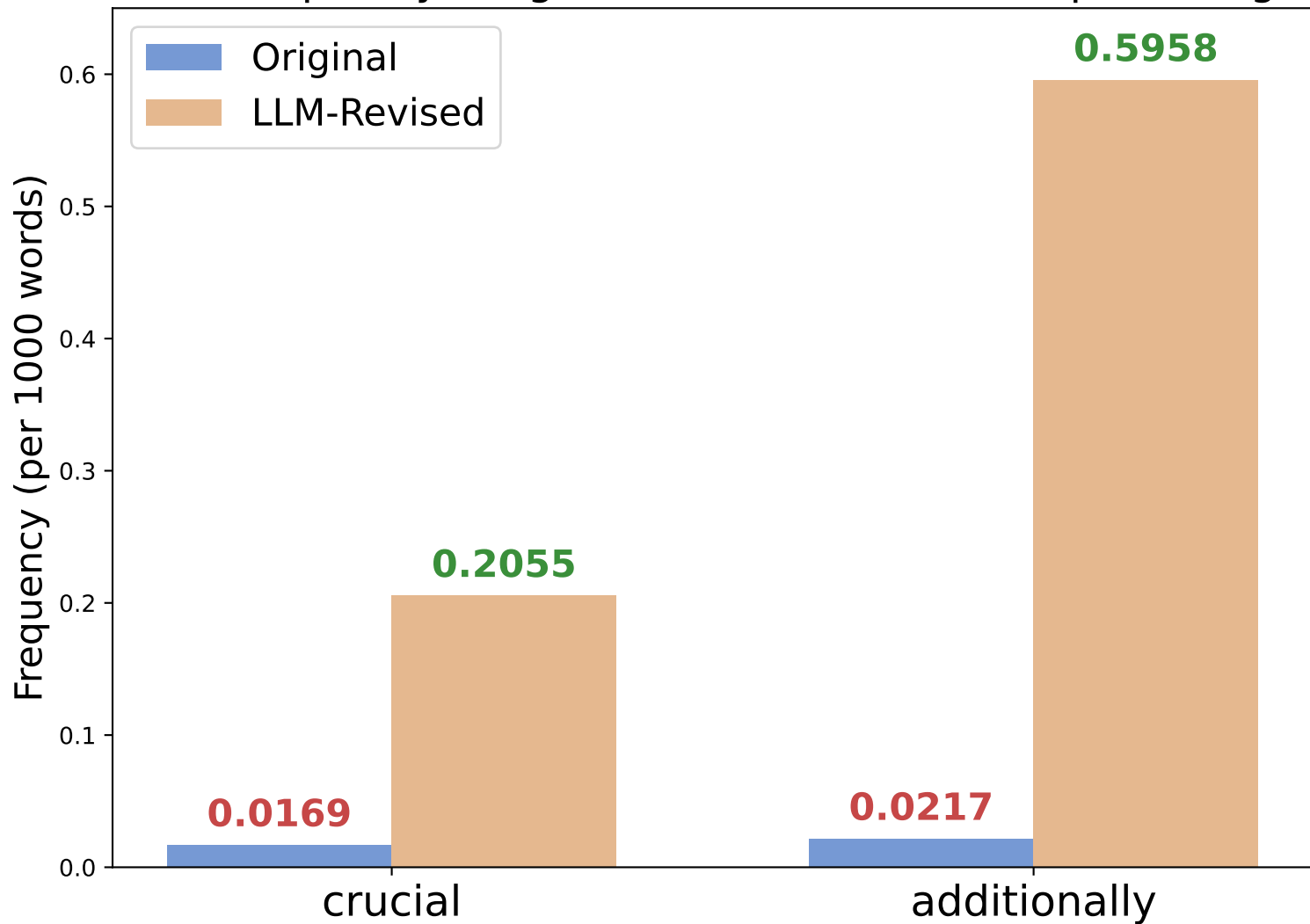
Word Frequency: Original vs LLM-Revised Wikipedia Pages
