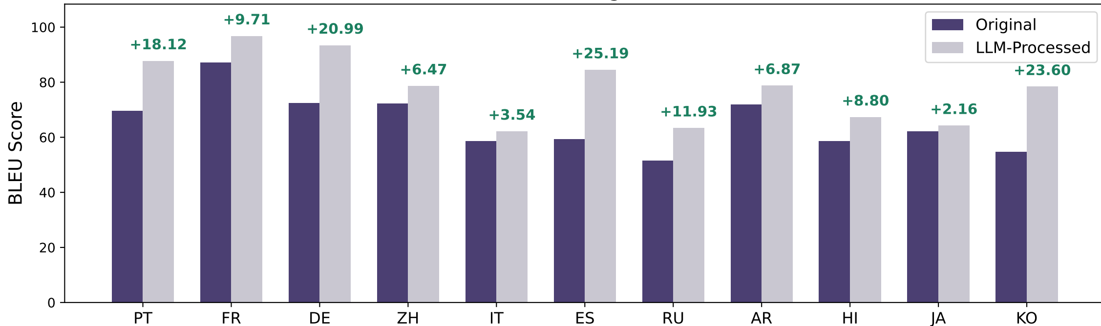
Facebook-NLLB BLEU Performance on Original vs LLM-Influenced Benchmarks
