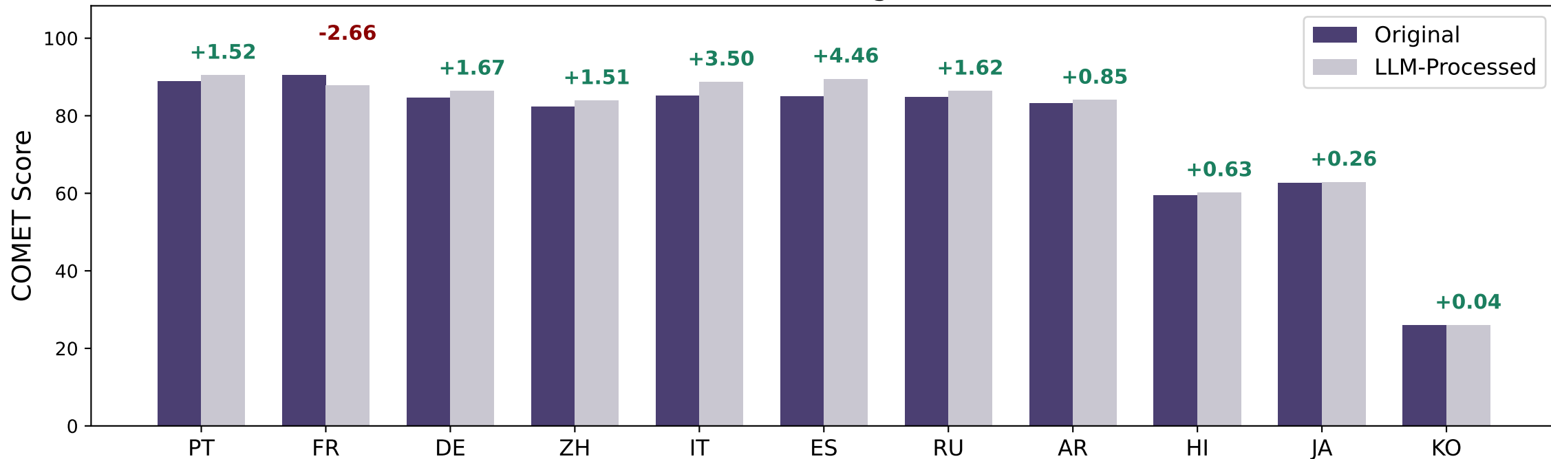
Facebook-NLLB COMET Performance on Original vs LLM-Influenced Benchmarks
