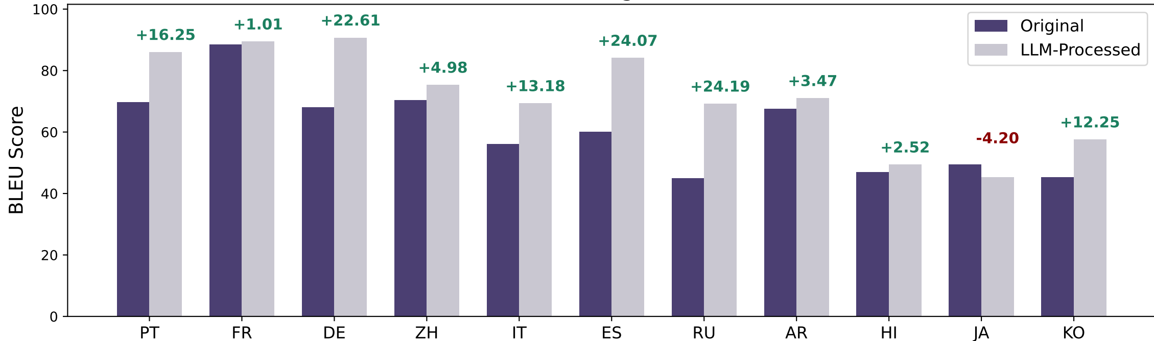
Helsinki-NLP BLEU Performance on Original vs LLM-Influenced Benchmarks
