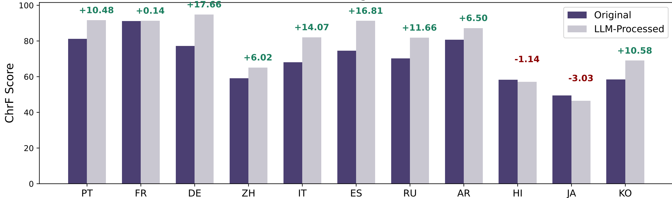
Helsinki-NLP ChrF Performance on Original vs LLM-Influenced Benchmarks
