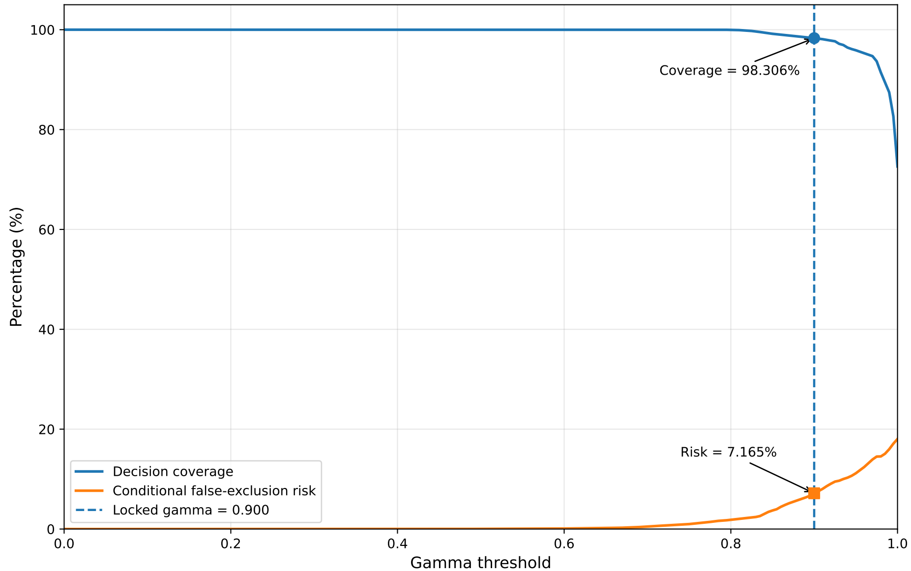
Gamma-sweep decision coverage and conditional risk
