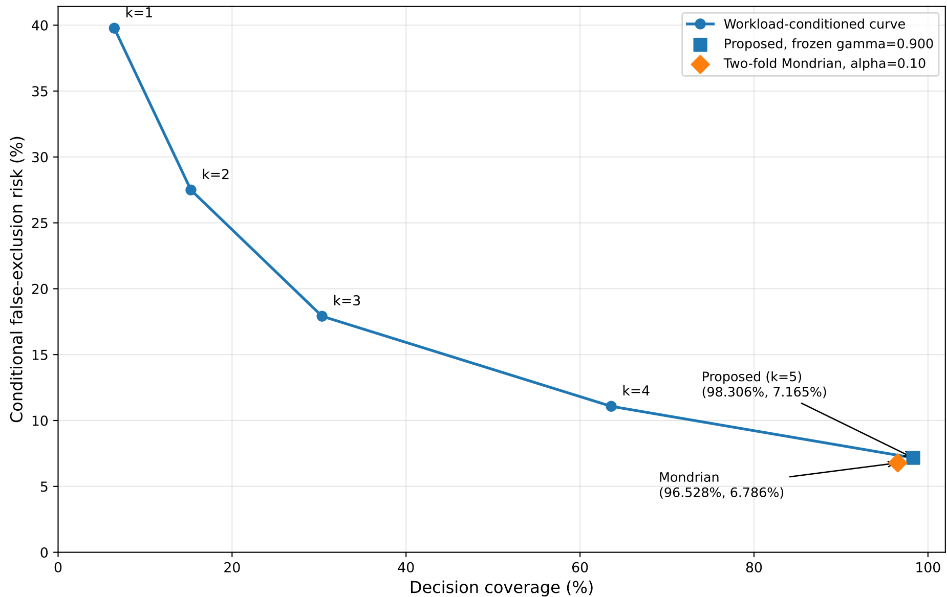
Workload-conditioned risk-coverage diagnostic
