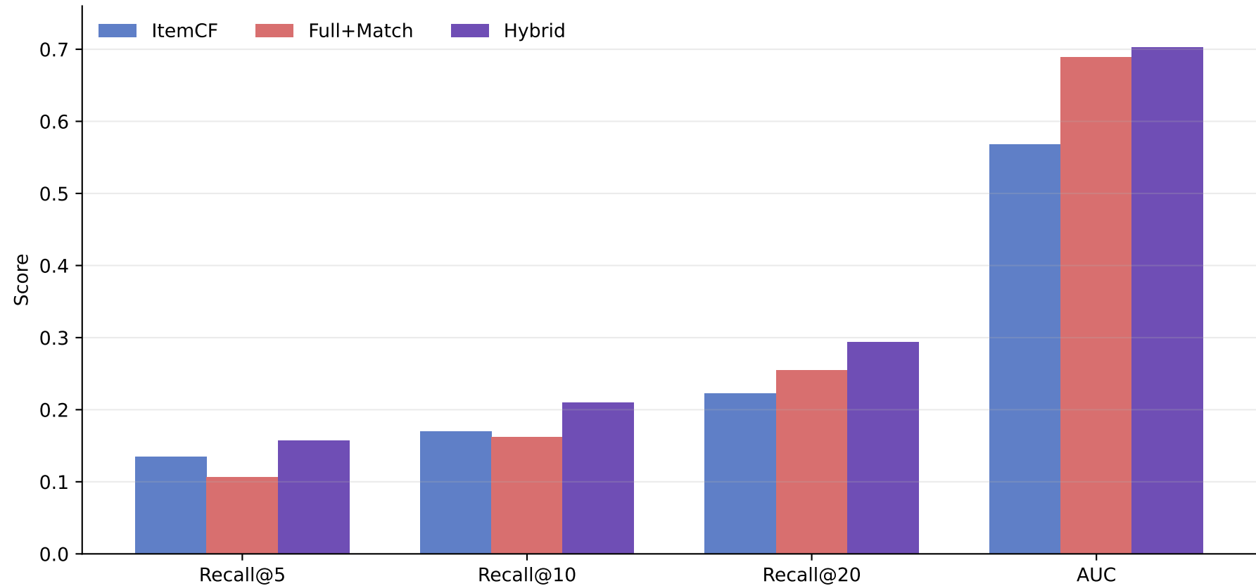
Complementarity of CF and Dynamic KG Signals
