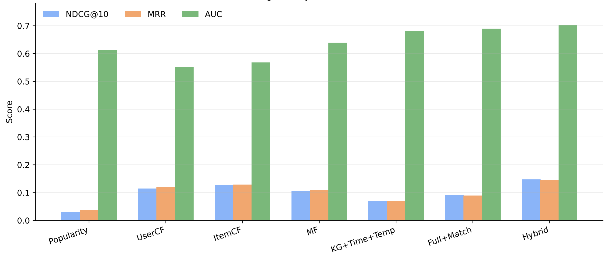
Ranking Quality and Discrimination
