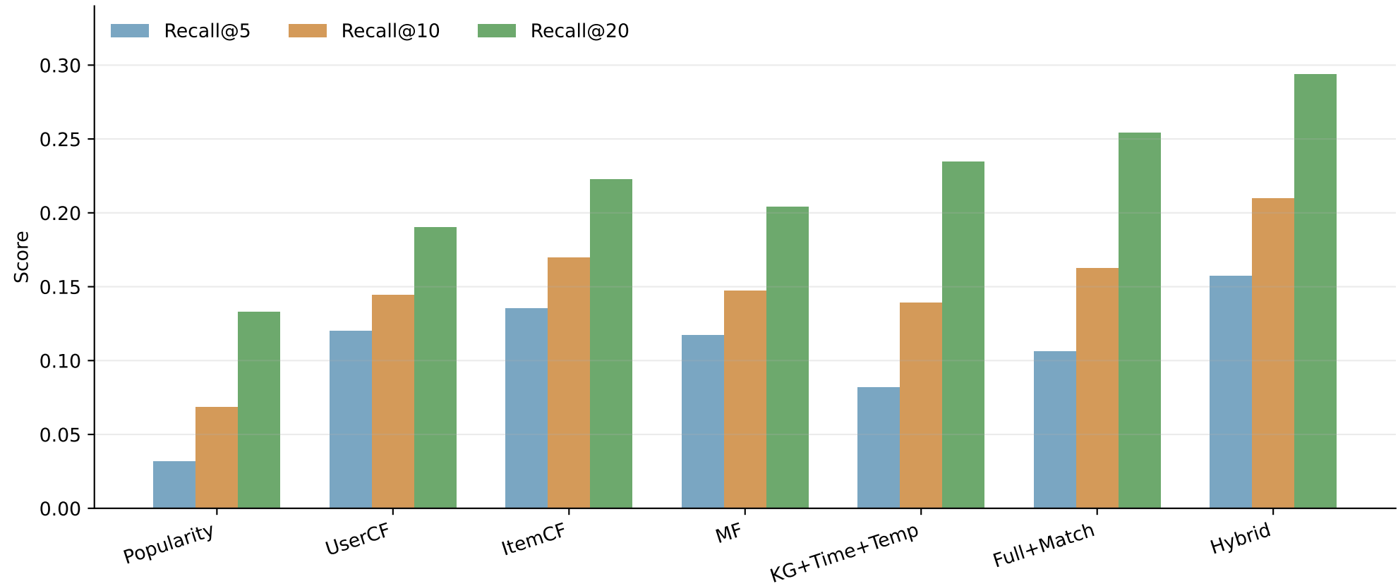
Sampled Recall@K Comparison
