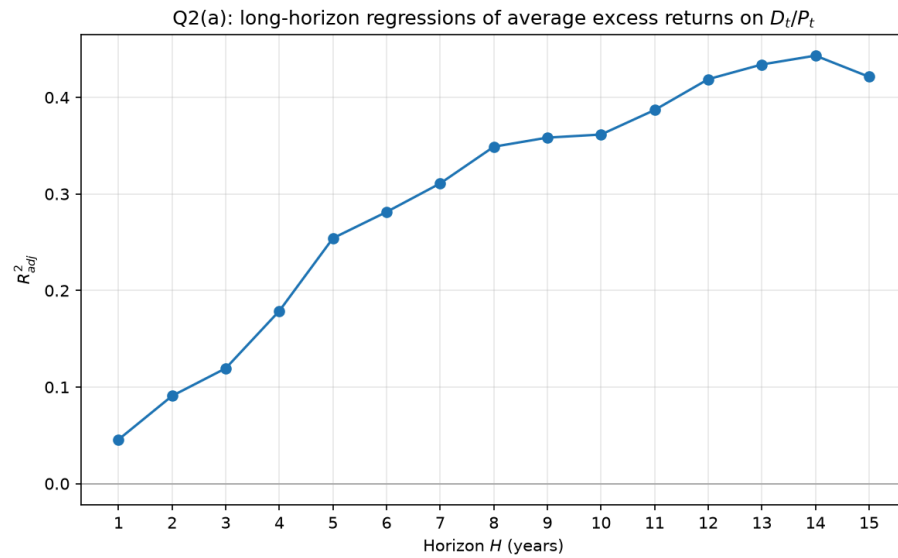
Figure 3: Adjusted R^2 of the Equation 2.1 regressions of the average future excess equity return \frac{1}{H} \sum_{h=1}^H x R_{e,t+h} on D_t/P_t , plotted against the horizon H = 1, \dots, 15 years (EQ Dataset, 1927:12–2021:12; overlapping monthly start dates, with year h taken 12h months ahead, so horizon H uses N - 12H observations).
