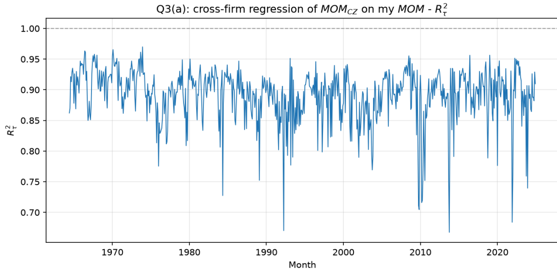
Figure 10: Monthly R_{\tau}^2 .
