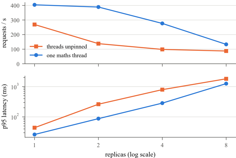
Replica scaling on one host, eight clients per replica
