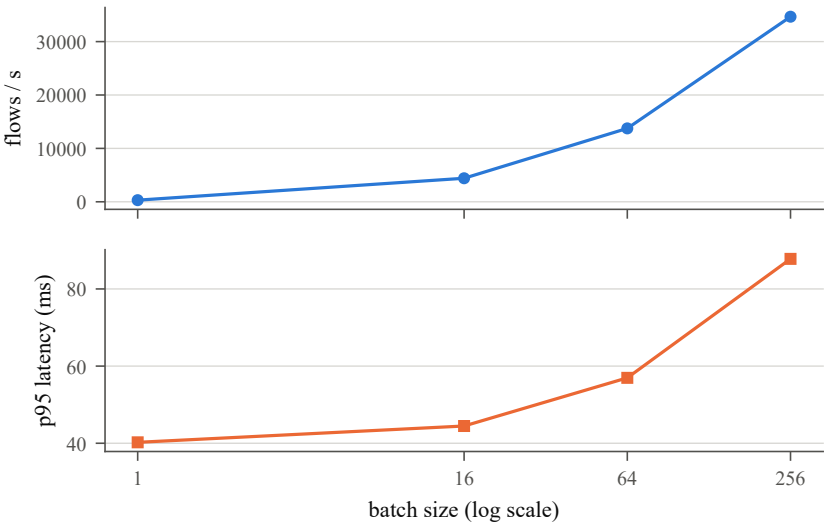
Batching trades latency for throughput
