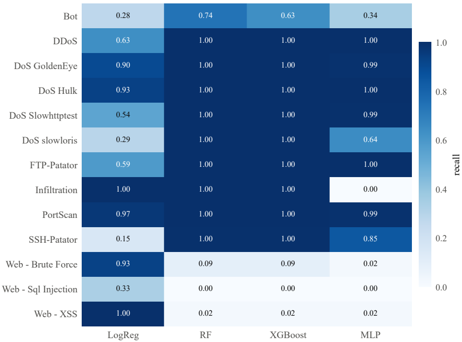
Per-family recall, random split
