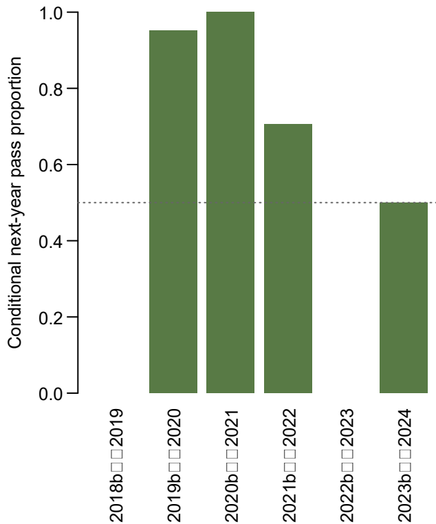
a Conditional next-year performance
