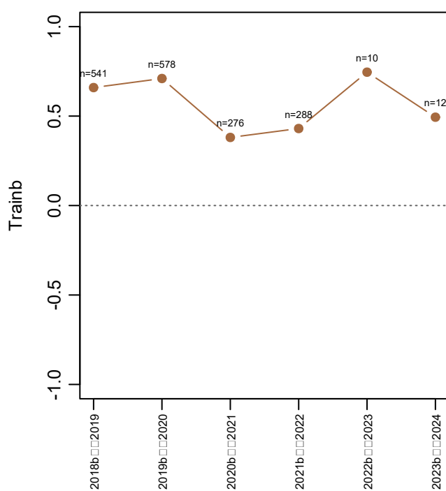
b Rank transportability
