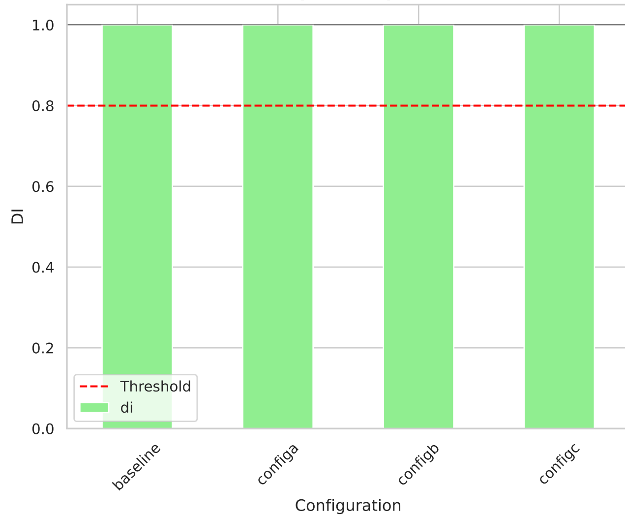
Disparate Impact
