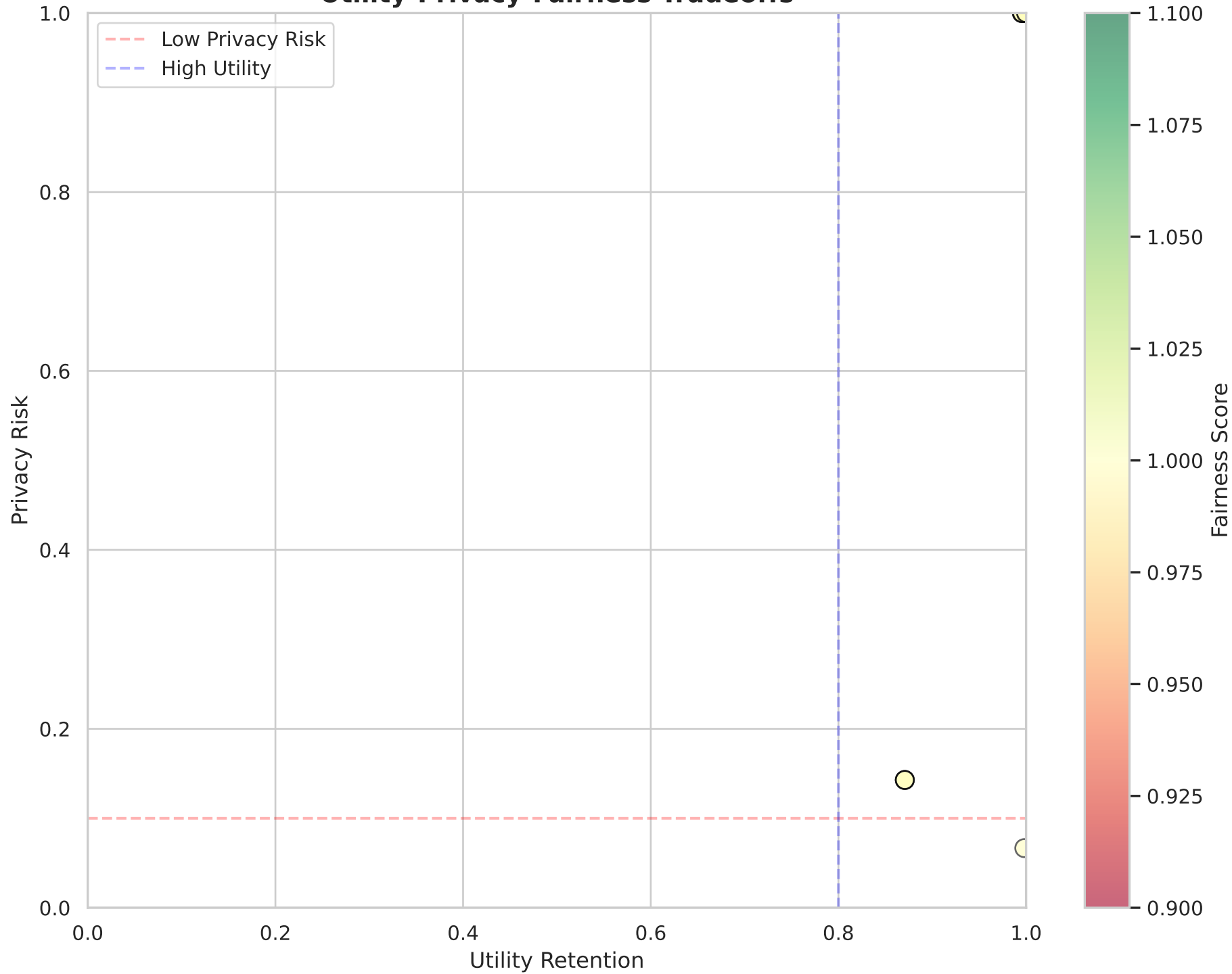
Utility-Privacy-Fairness Tradeoffs
