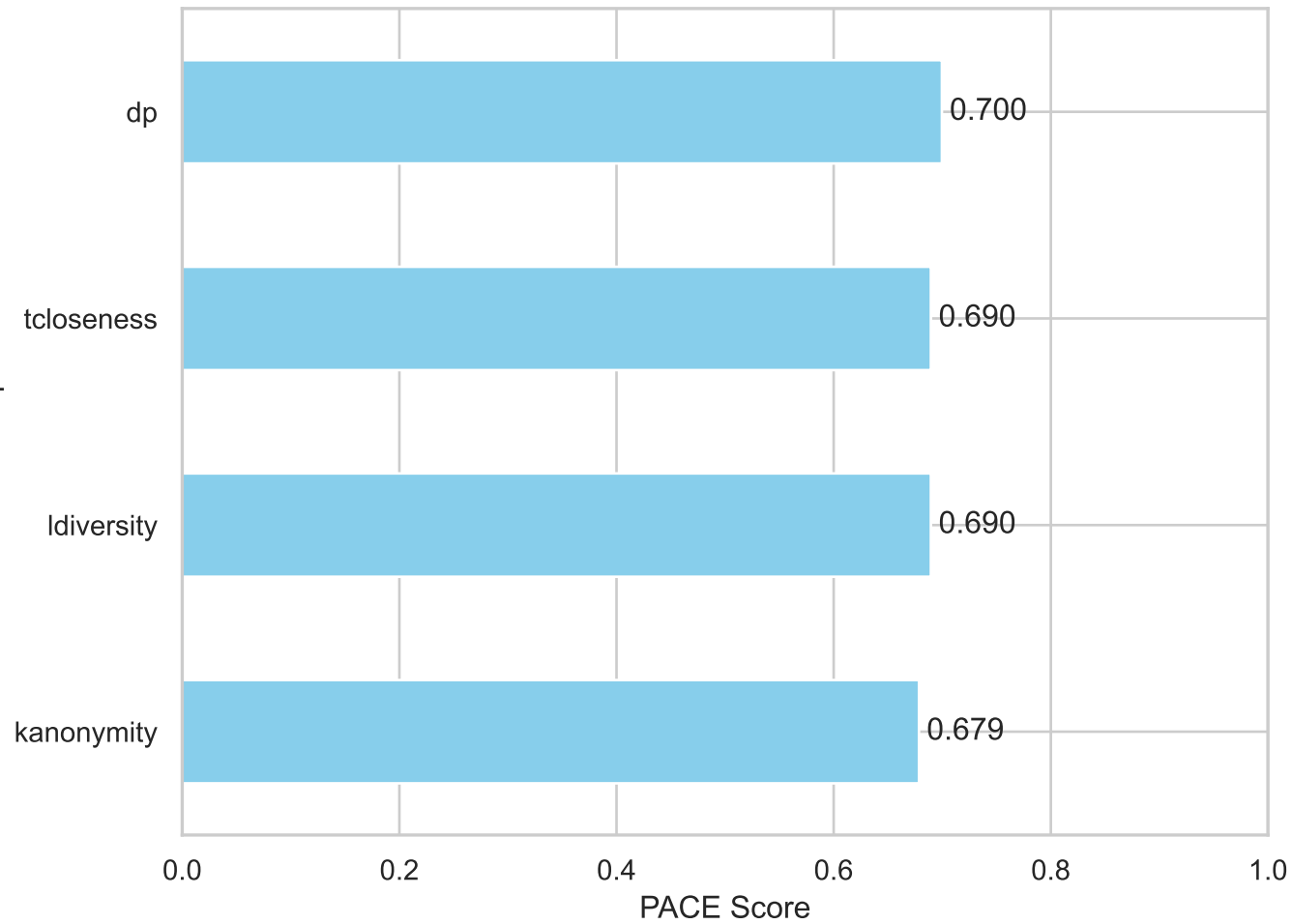
PACE Score by Technique
