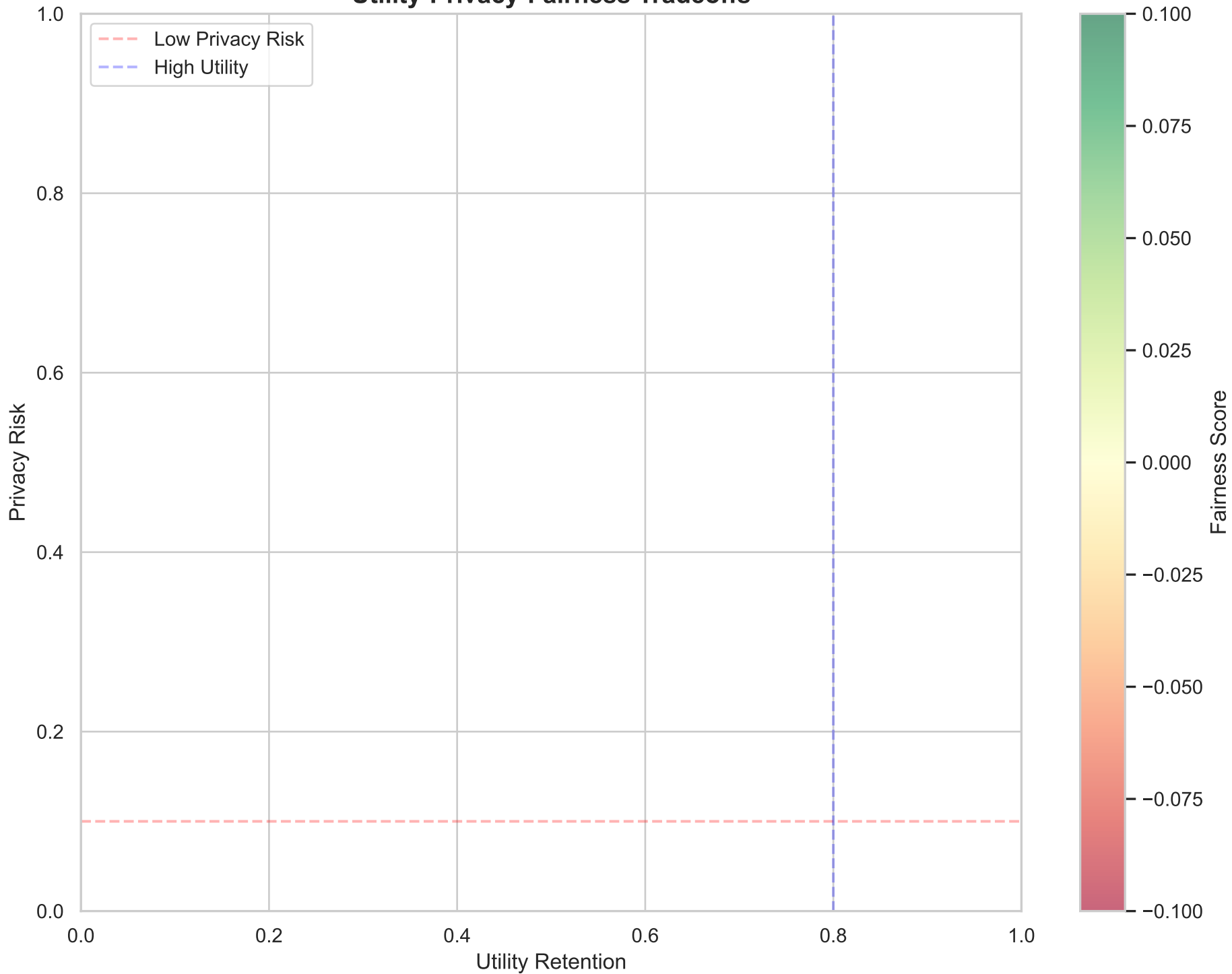
Utility-Privacy-Fairness Tradeoffs
