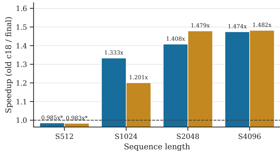
Head dimension D=64
