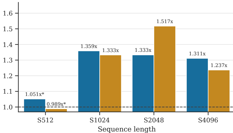
Head dimension D=128
