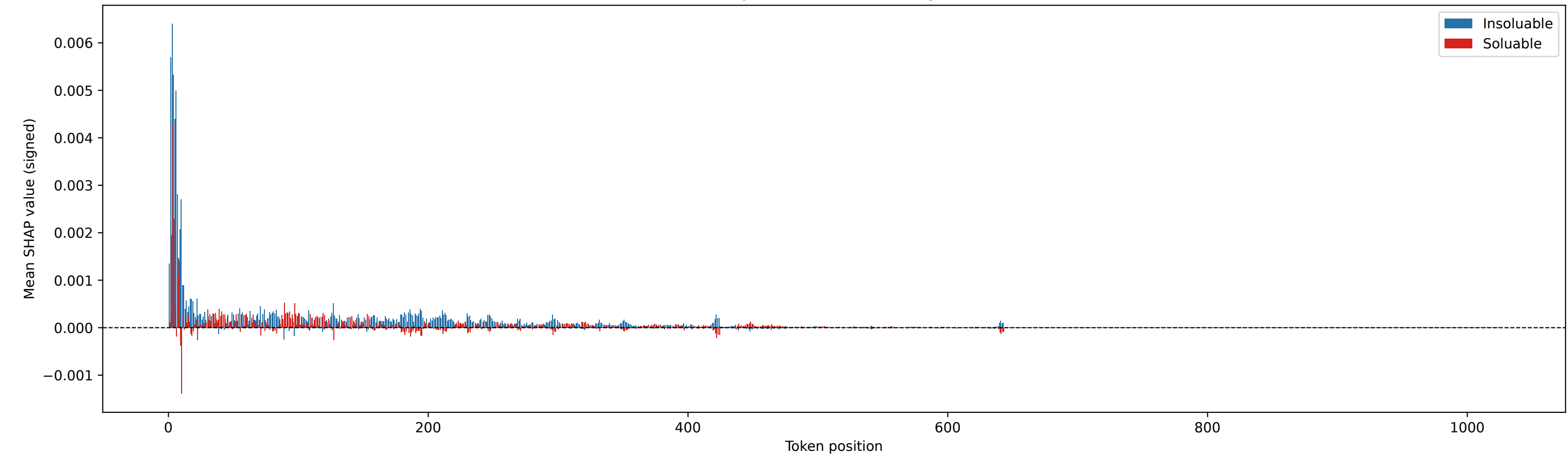
SynCodonLM Embedding
