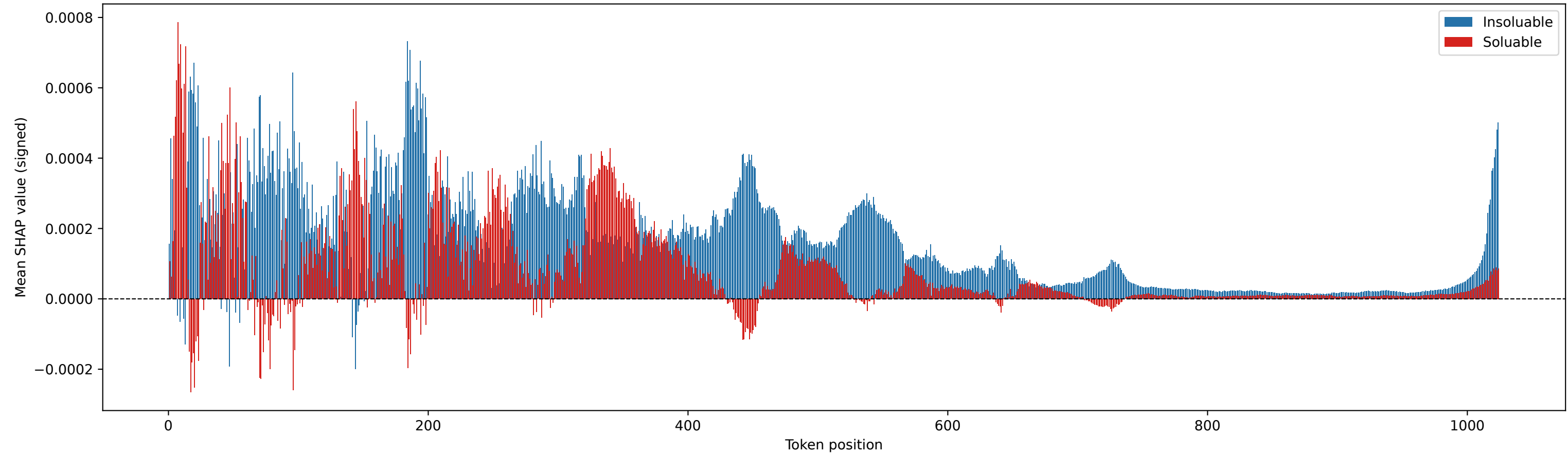
SynCodonLM Embedding
