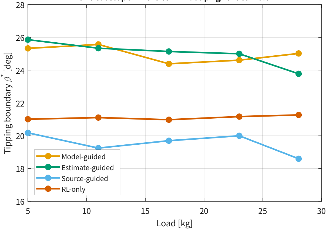
C2 Anti-tipping boundary \beta^* (load) critical slope where terminal upright-rate < 0.5
